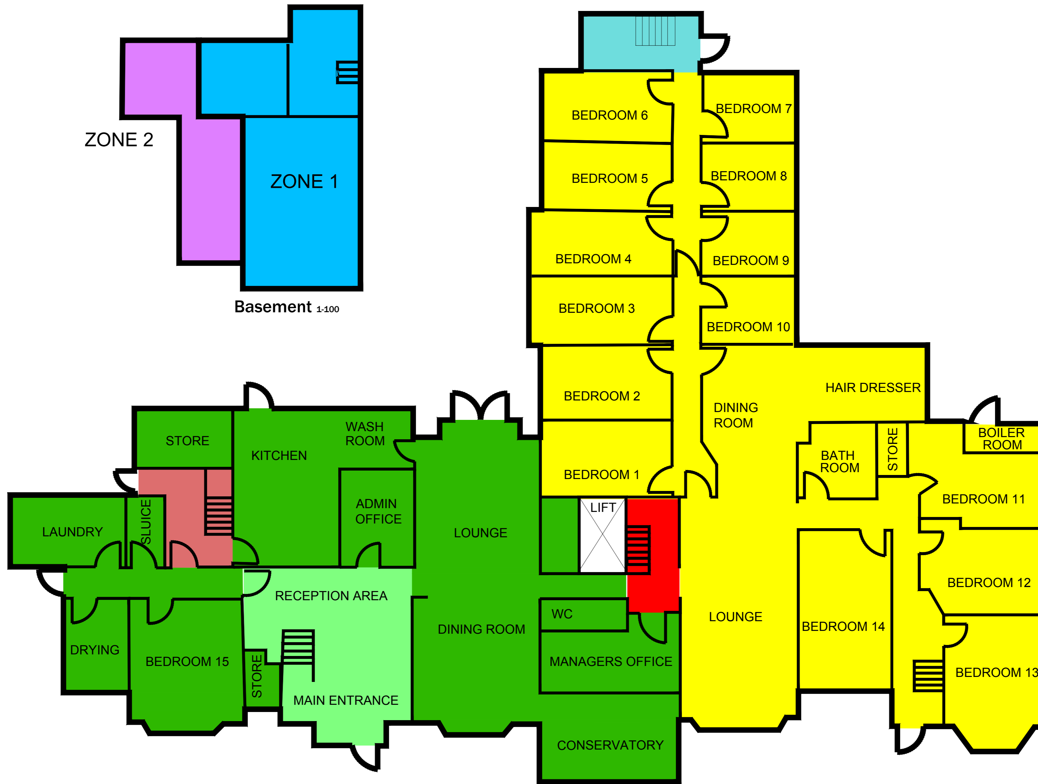
Ground Floor 1-100
